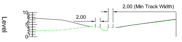
Powdermill Cross Section 5 - 5 SCALE: H 1:500, V 1:500. DATUM: 0.000
